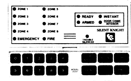
MODEL 2090 REMOTE MODULE
